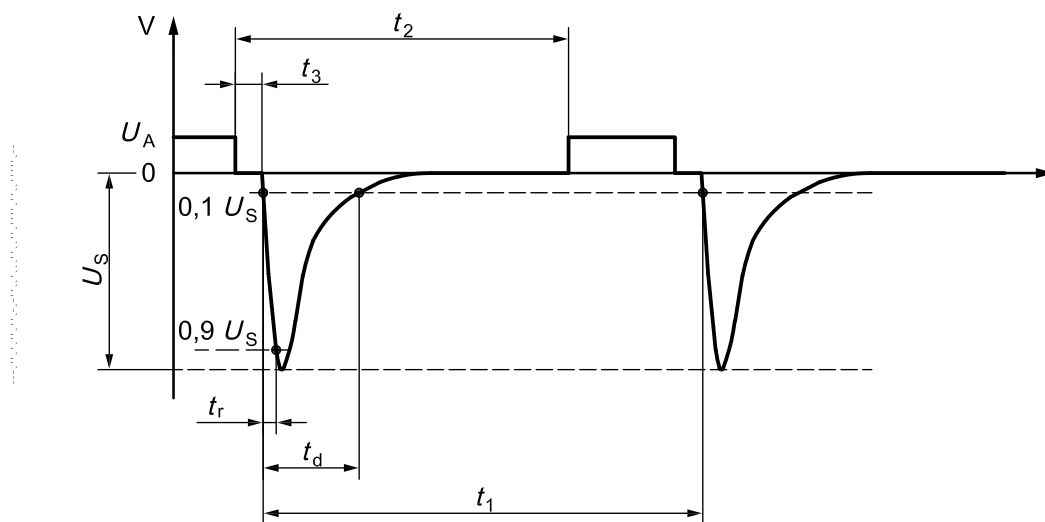
Figure 5 — Test pulse 1
