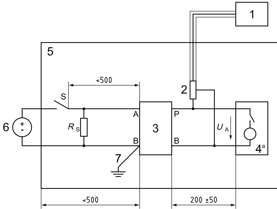
a) Transient emission test set-up to measure slow pulses (ms-range or slower)
